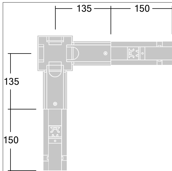
TL_CONTUS_M_L4_Node_Connector.wmf
